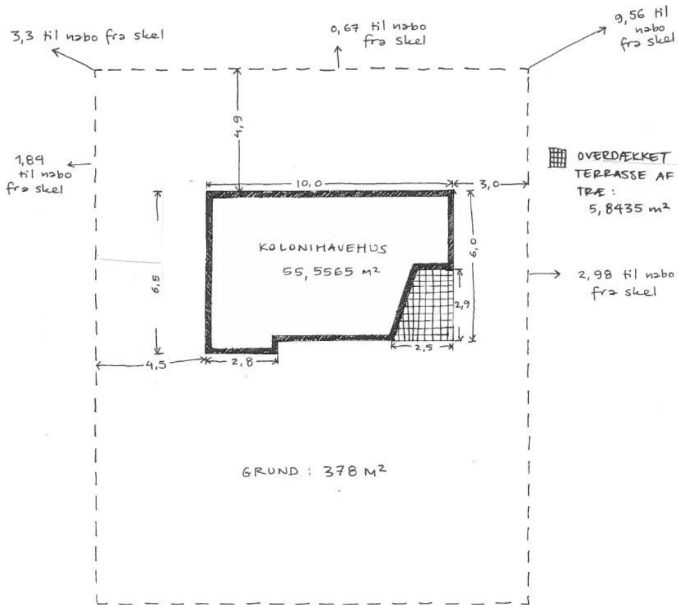
1:125 Situationsplan
